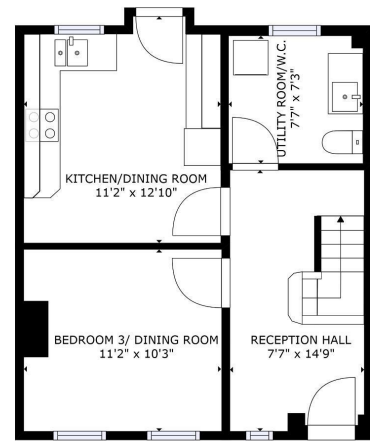
GROSS INTERNAL AREA FLOOR 1: 434 SQ. FT. FLOOR 2: 432 SQ. FT. TOTAL: 866 SQ. FT. NOTE: AREA SHOWN IS FOR APPROXIMATE ACTUAL SIZE ONLY.
