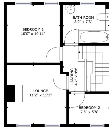
GROSS INTERNAL AREA FLOOR 1: 434 SQ. FT. FLOOR 2: 432 SQ. FT. TOTAL: 866 SQ. FT. NOTE: AREA SHOWN IS FOR APPROXIMATE ACTUAL SIZE ONLY.
