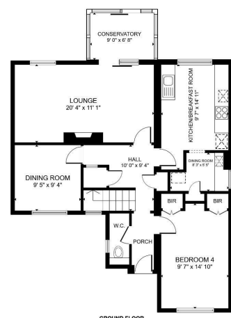
GROUND FLOOR GROSS INTERNAL AREA GROUND FLOOR 888 sq ft FLOOR 1 560 sq ft TOTAL 1,448 sq ft *BASED ON CONVENTIONAL BUILDING STANDARDS, ACTUAL MAY VARY
