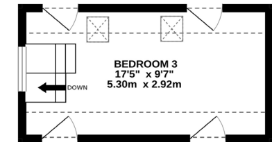
2ND FLOOR 167 sq.ft. (15.5 sq.m.) approx.
