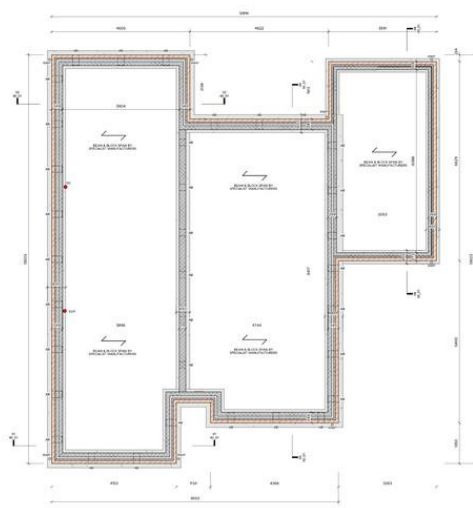
01 Below Ground Floor Plan Scale 1:50
