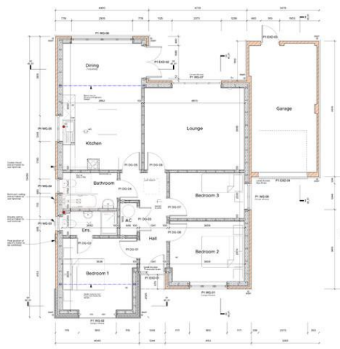
02 Ground Floor Plan Scale: 1:50
