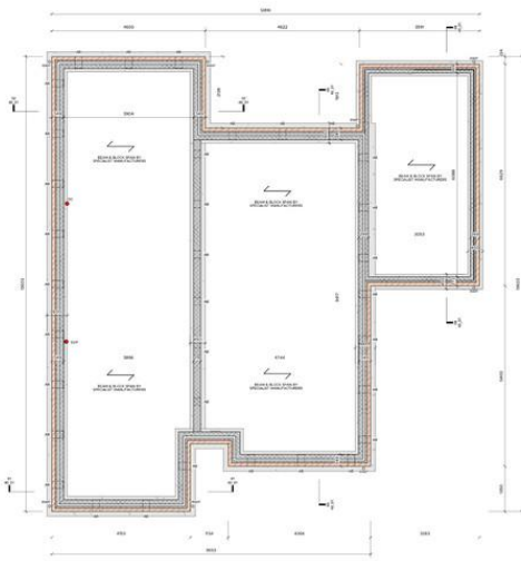
01 Below Ground Plan Scale: 1:50
