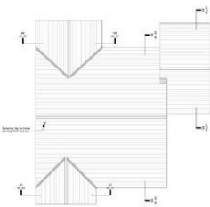
03 Roof Plan Scale: 1:50
