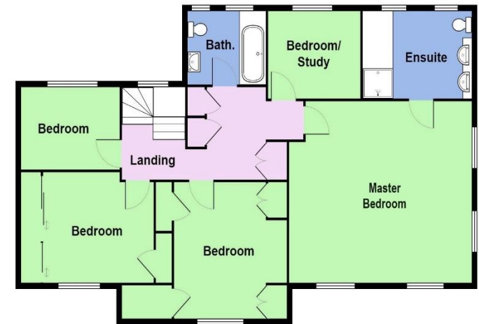
1st Floor Area: 95.9 m 2 ... 1032 ft 2
