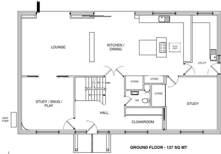
GROUND FLOOR - 127 SQ MT
