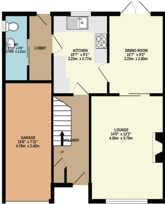
GROUND FLOOR 625 sq.ft. (58.0 sq.m.) approx.
