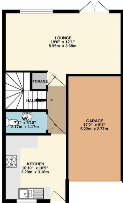
GROUND FLOOR 568 sq.ft. (52.8 sq.m.) approx.
