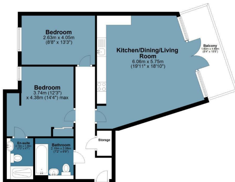
Second Floor Approx. 69.1 sq. metres (743.8 sq. feet)
