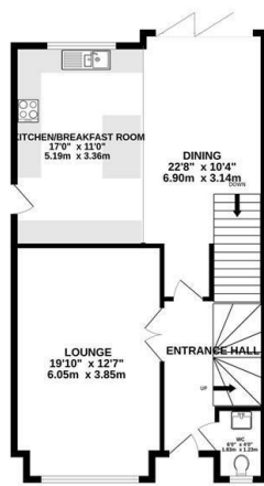
GROUND FLOOR 783 sq.ft. (72.8 sq.m.) approx.
