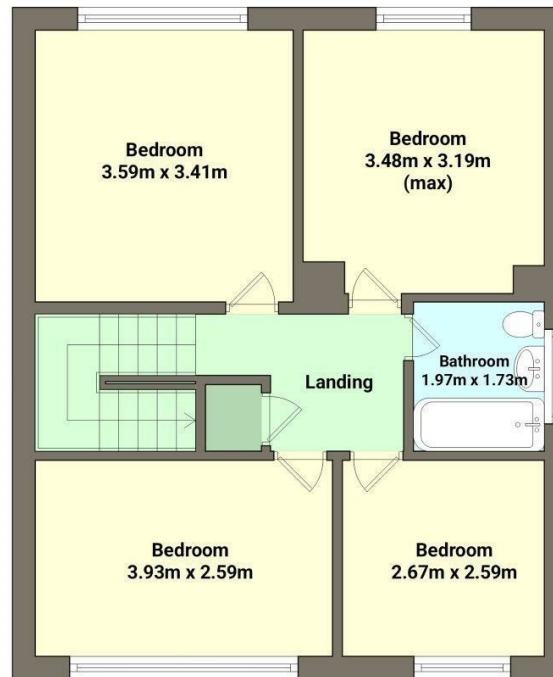
First floor Area: 51.94 m 2
