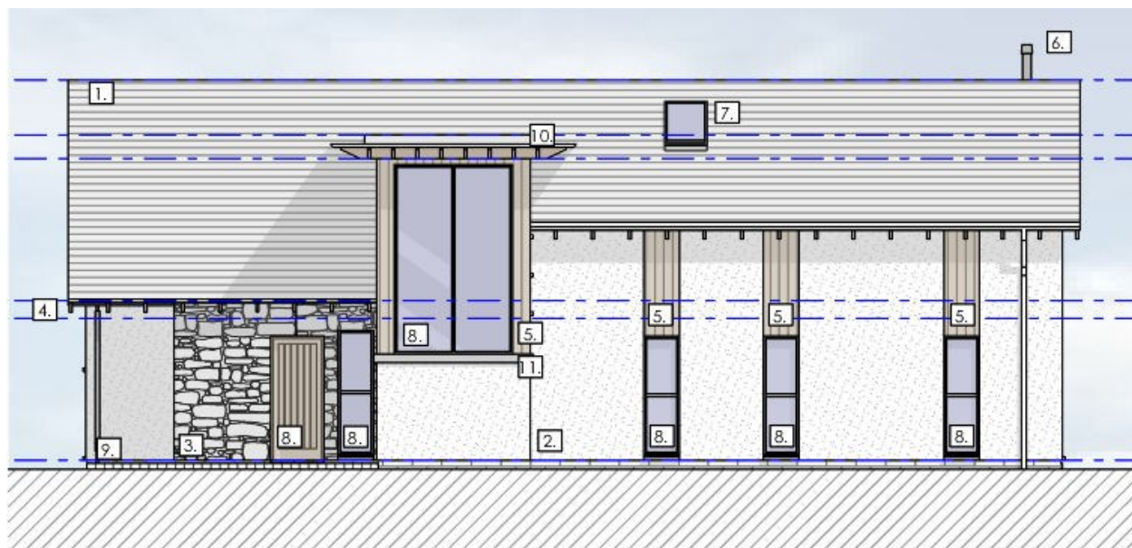
Proposed North Elevation Plan - scale 1:100
