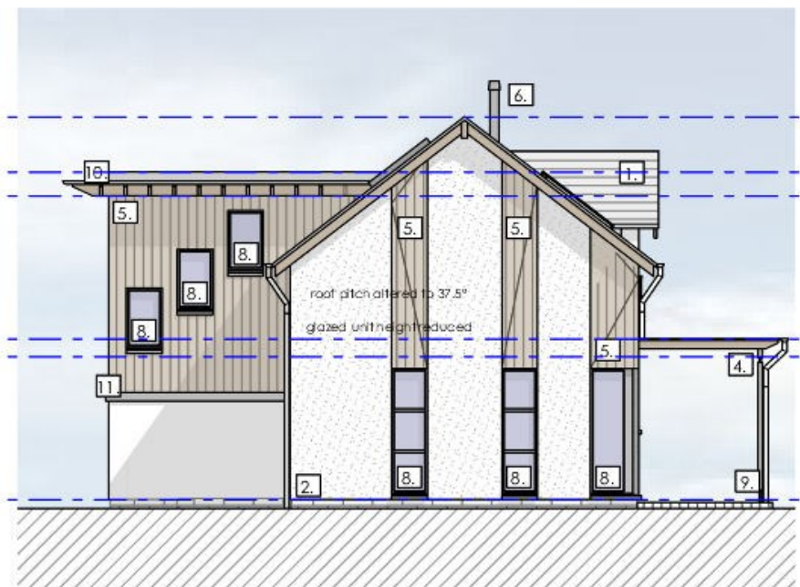
Proposed West Elevation Plan - scale 1:100
