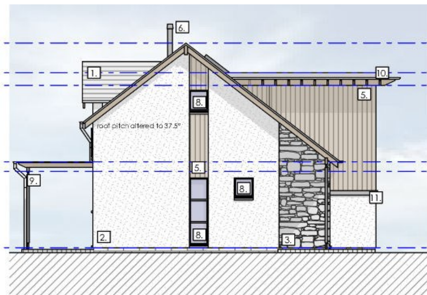
Proposed East Elevation Plan - scale 1:100
