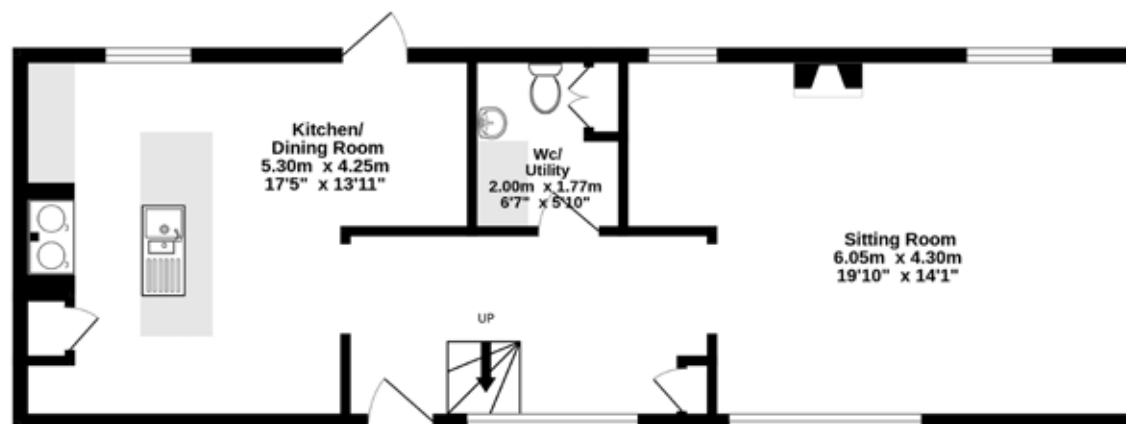
Ground Floor 55.9 sq.m. (601 sq.ft.) approx.
