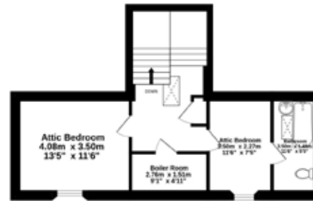
3rd Floor 98.6 sq.m. (1062 sq.ft.) approx.
