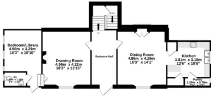
Basement 60.0 sq.m. (648 sq.ft.) approx.
