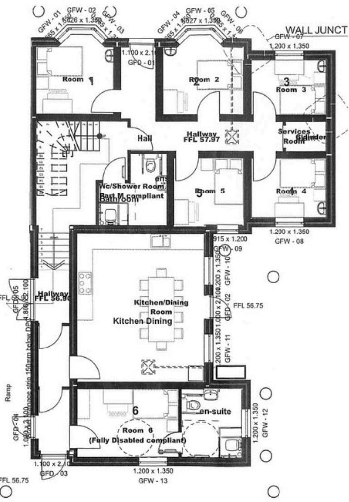
GROUND FLOOR 1:100
