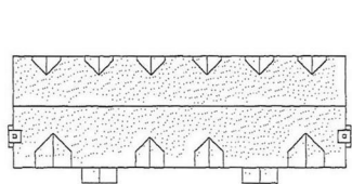
Roof Plan
