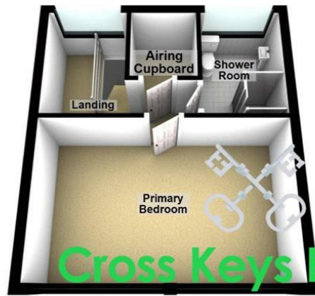
Split Level Second Floor
