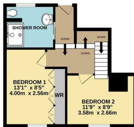
1ST FLOOR 367 sq.ft. (34.1 sq.m.) approx.
