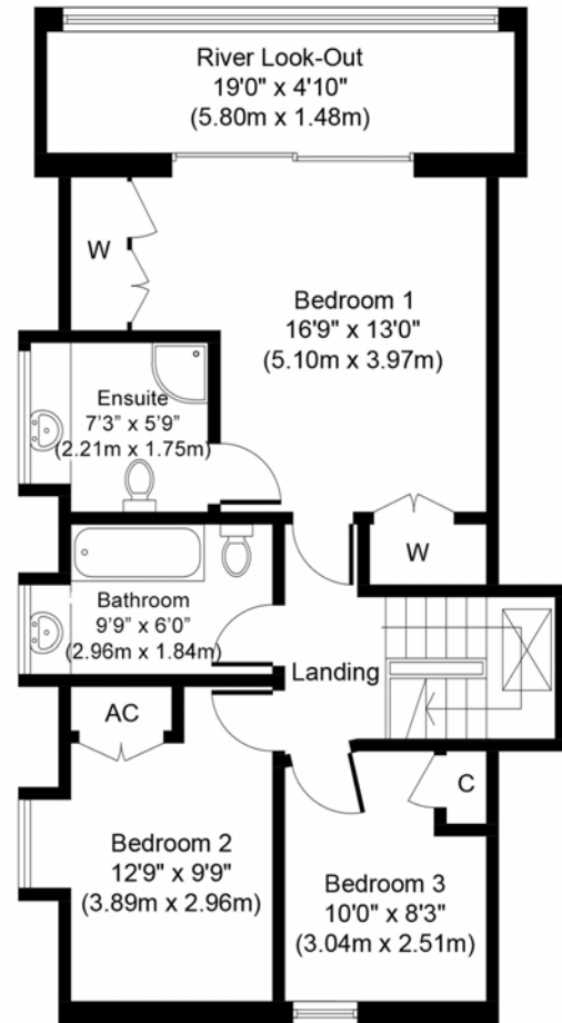
First Floor Approximate Floor Area 713 Sq. ft. (66.2 Sq. m.)
