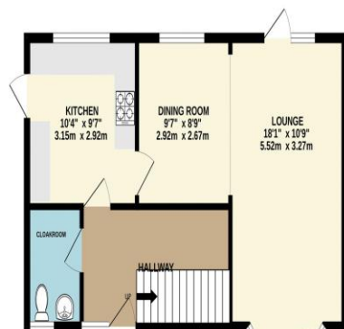
GROUND FLOOR 791 sq.ft. (73.5 sq.m.) approx.
