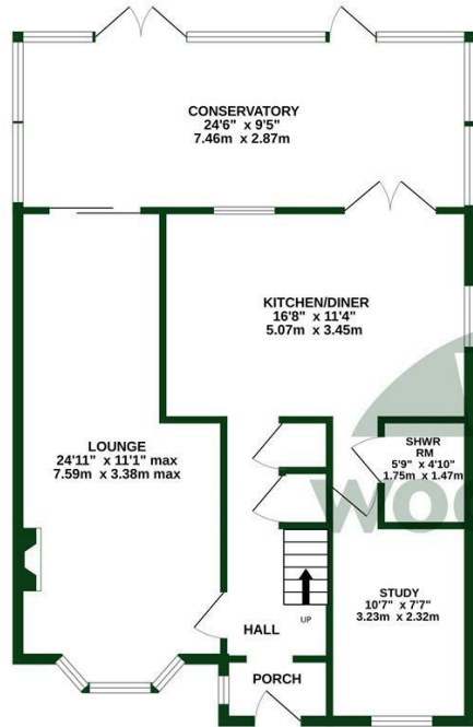
GROUND FLOOR 876 sq.ft. (81.4 sq.m.) approx.
