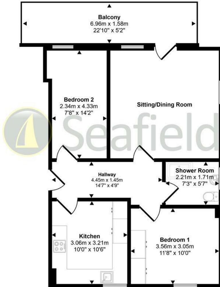
Floorplan
