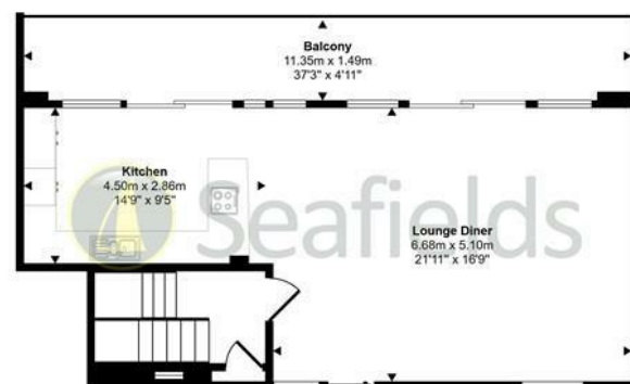
First Floor Approx 55 sq m / 589 sq ft
