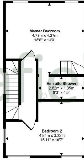
Second Floor Approx 44 sq m / 473 sq ft
