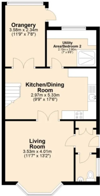
Ground Floor Approx. 50.9 sq. metres (548.1 sq. feet)
