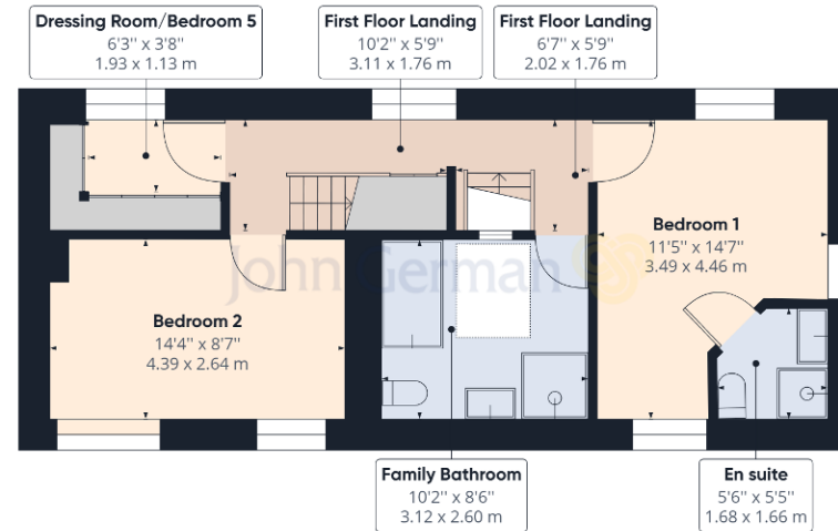
Floor 1 Building 1
