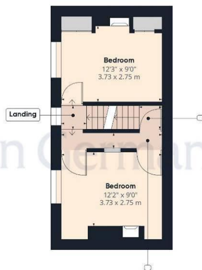
Floor 2 Building 1
