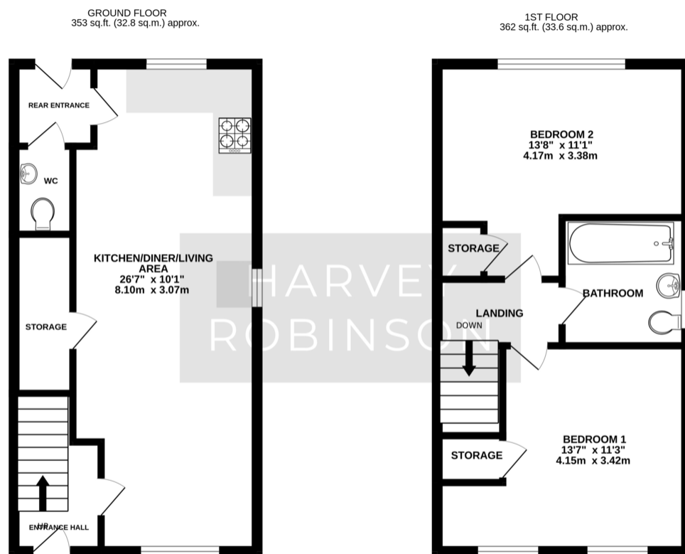
TOTAL FLOOR AREA : 715 sq.ft. (66.4 sq.m.) approx. Made with Metropix ©2024
