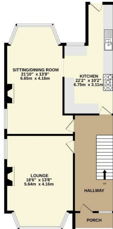
GROUND FLOOR 860 sq.ft. (79.9 sq.m.) approx.
