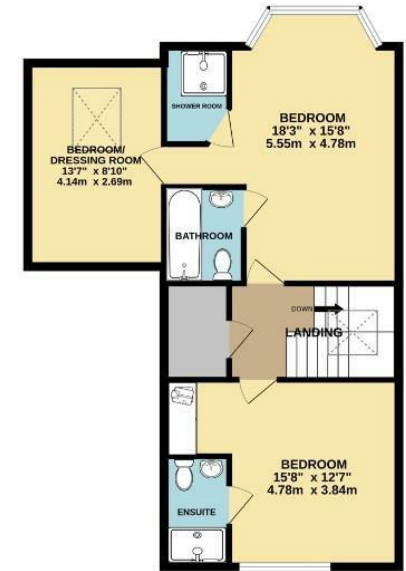
2ND FLOOR 686 sq.ft. (63.7 sq.m.) approx.
