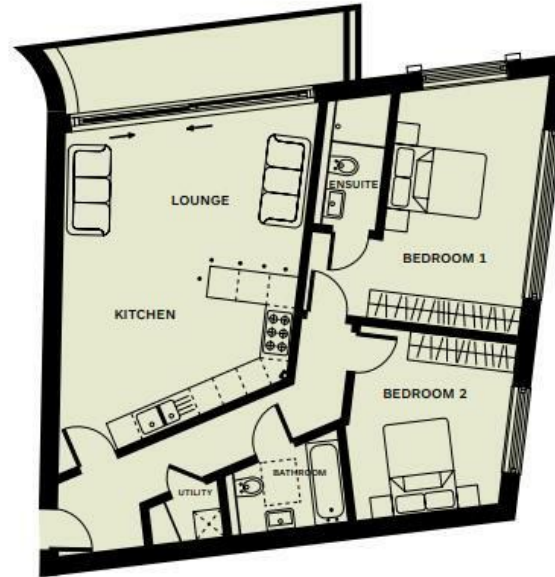
APARTMENT 6 - 922 SQ.FT.
