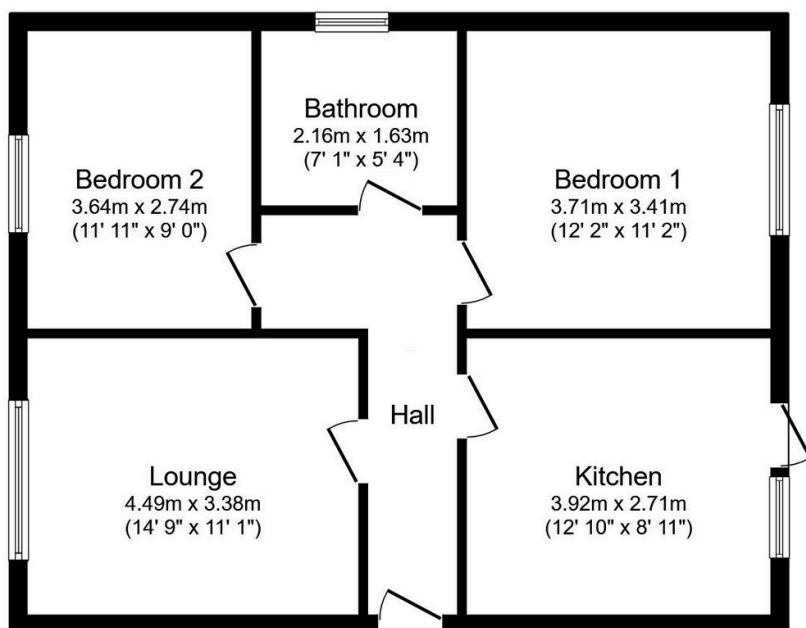
Floor Plan
