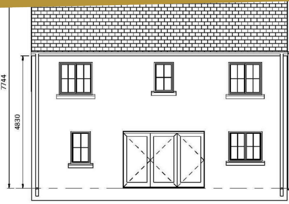
3 Rear Elevation 1 : 50
