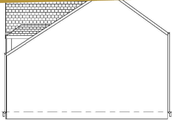
4 Right Side Elevation 1 : 50
