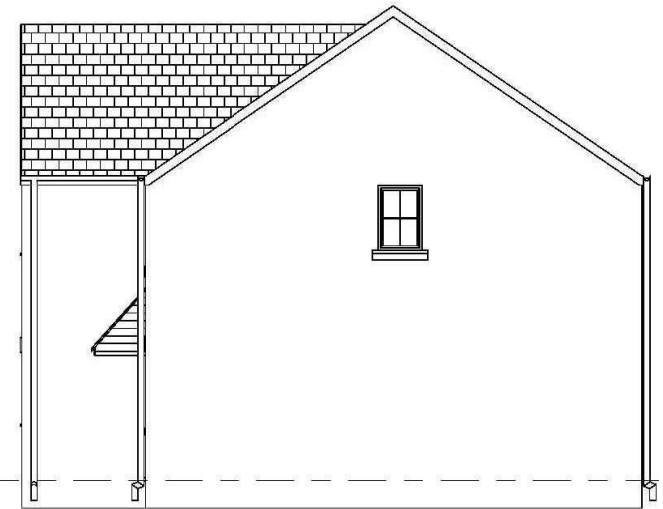
4 Right Side Elevation 1 : 50
