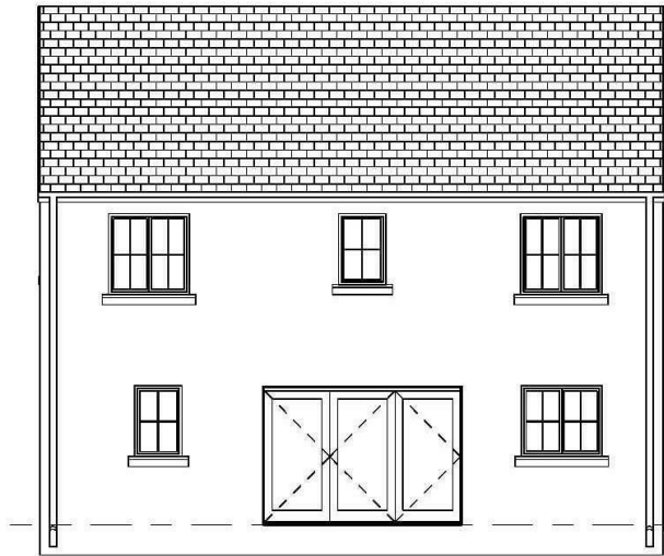
3 Rear Elevation 1 : 50
