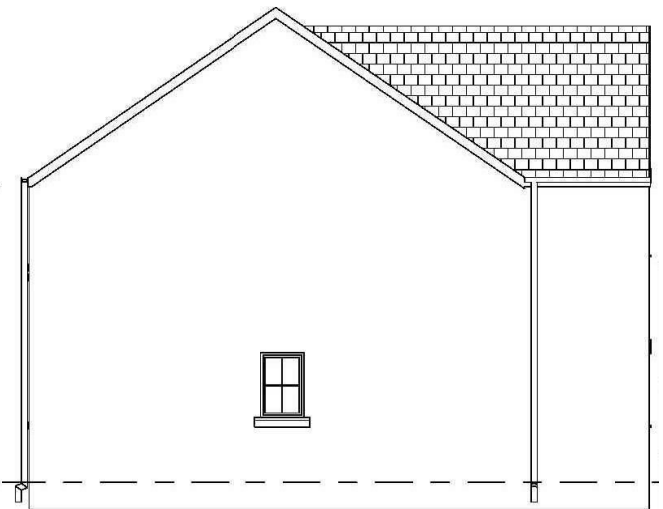
6 Left Side Elevation 1 : 50
