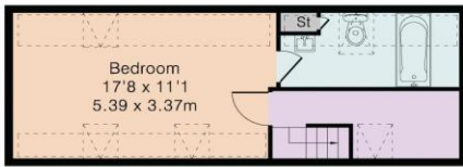
Annexe First Floor
