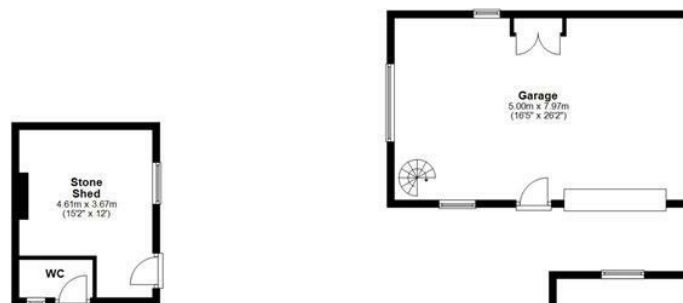
Ground Floor Approx. 208.9 sq. metres (2240.9 sq. feet)
