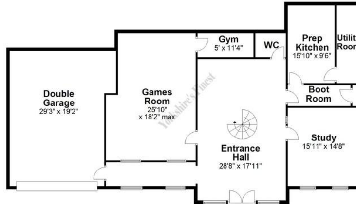
Ground Floor Approx. 2588.5 sq. feet
