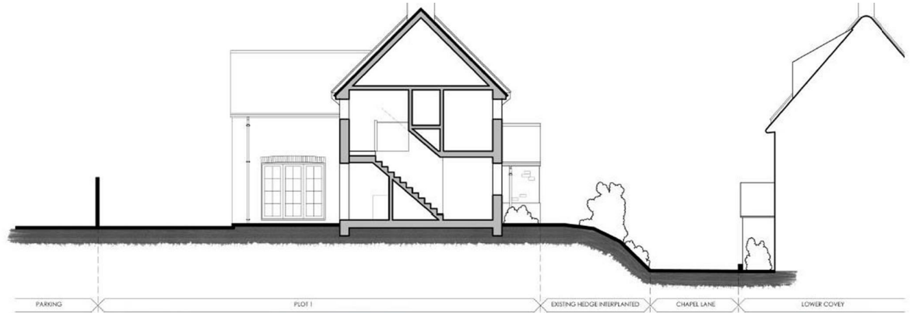
SITE SECTION AA (proposed) - scale 1/100
