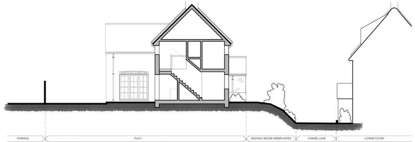
SITE SECTION AA (proposed) - scale 1/100 0 2m 4m
