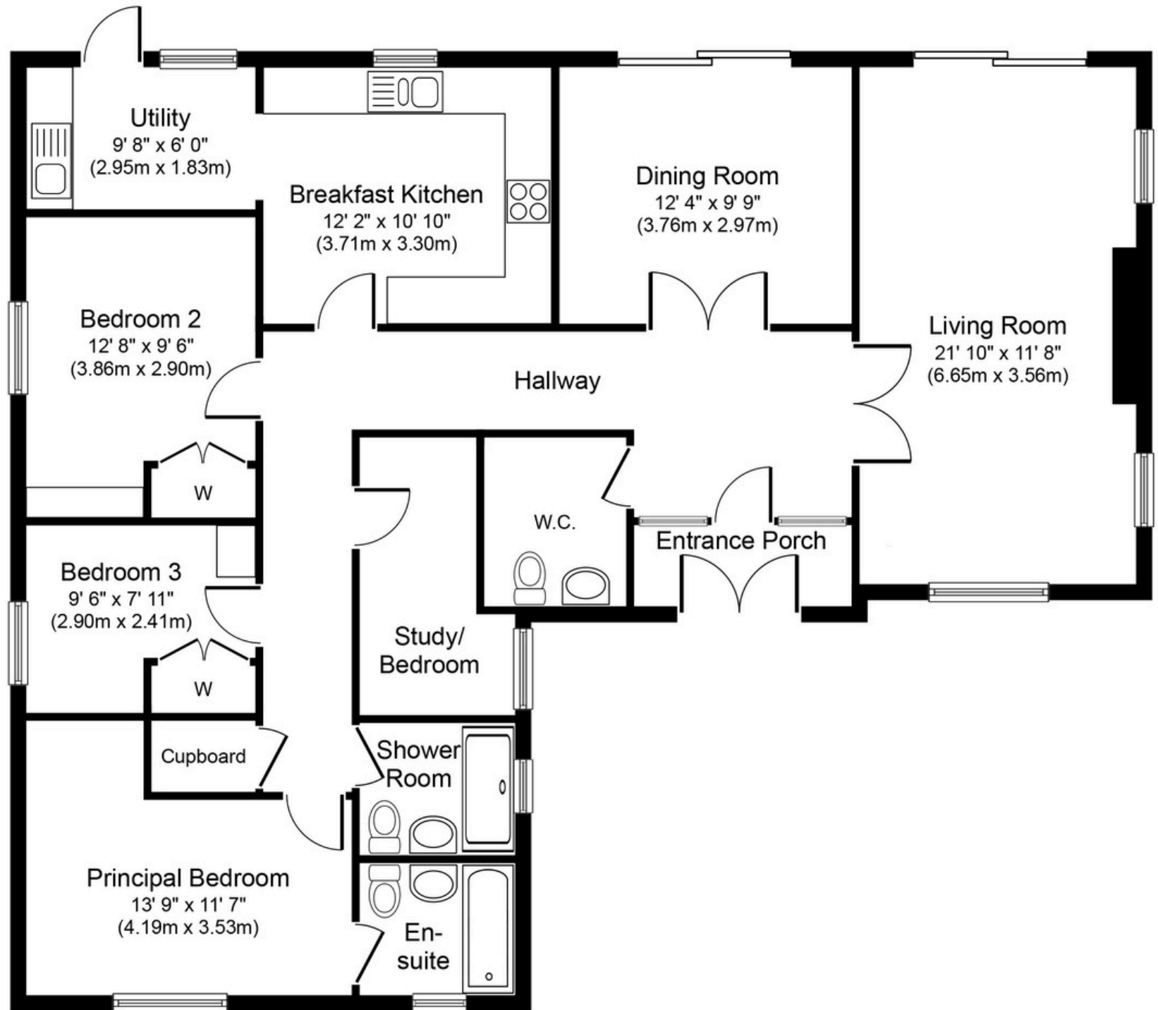
Ground Floor Approximate Floor Area 1,394 sq. ft. (129.5 sq. m.)
