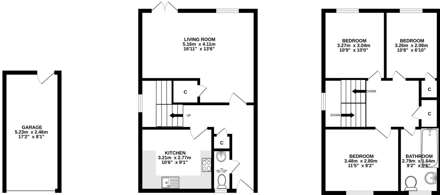
TOTAL FLOOR AREA : 94.6 sq.m. (1019 sq.ft.) approx.
