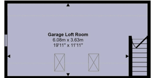
Garage First Floor Approx 26 sq m / 275 sq ft
