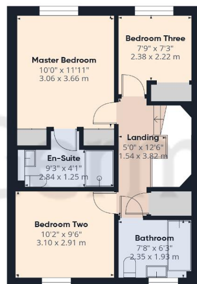
Floor 1
