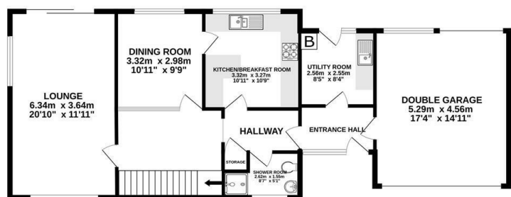
GROUND FLOOR 97.2 sq.m. (1046 sq.ft.) approx.
