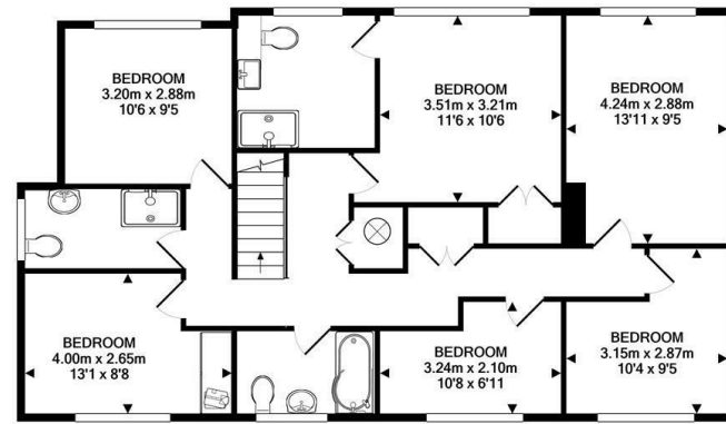
1ST FLOOR APPROX. FLOOR AREA 94.5 SQ.M. (1017 SQ.FT.)
