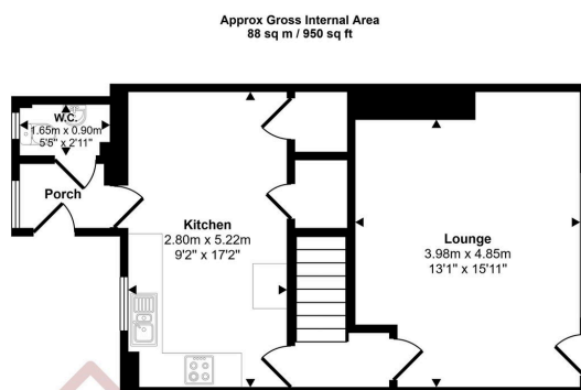
Ground Floor Approx 46 sq m / 500 sq ft
