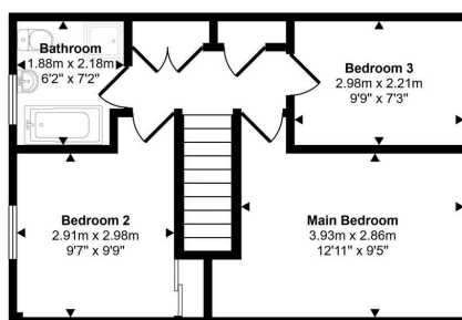
First Floor Approx 42 sq m / 450 sq ft
