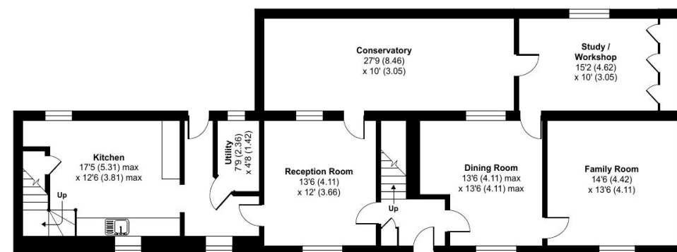
GROUND FLOOR
