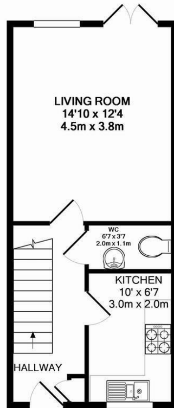
GROUND FLOOR APPROX. FLOOR AREA 350 SQ.FT. (32.5 SQ.M.)
