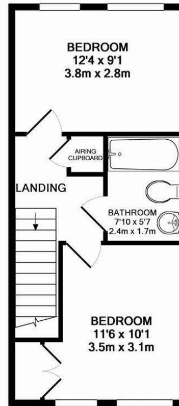
1ST FLOOR APPROX. FLOOR AREA 350 SQ.FT. (32.5 SQ.M.)
