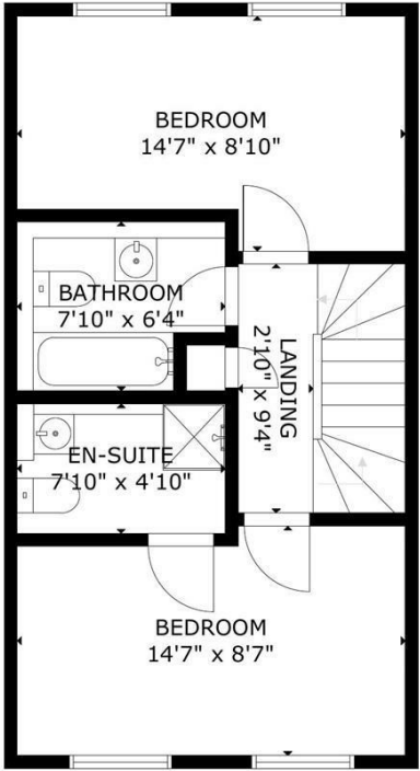
FLOOR 2
